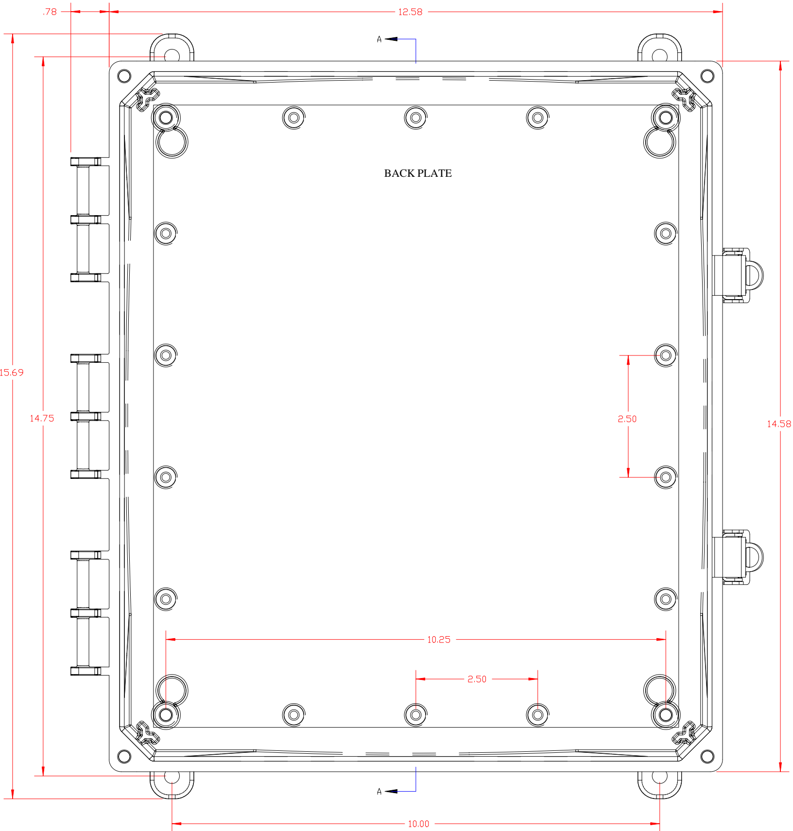
Inside View of EWP-14126 NEMA 4 Enclosure Electronic Security Devices www.SecurityPower.com
